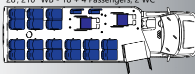
28', 210" WB - 18 + 4 Passengers, 2 WC
